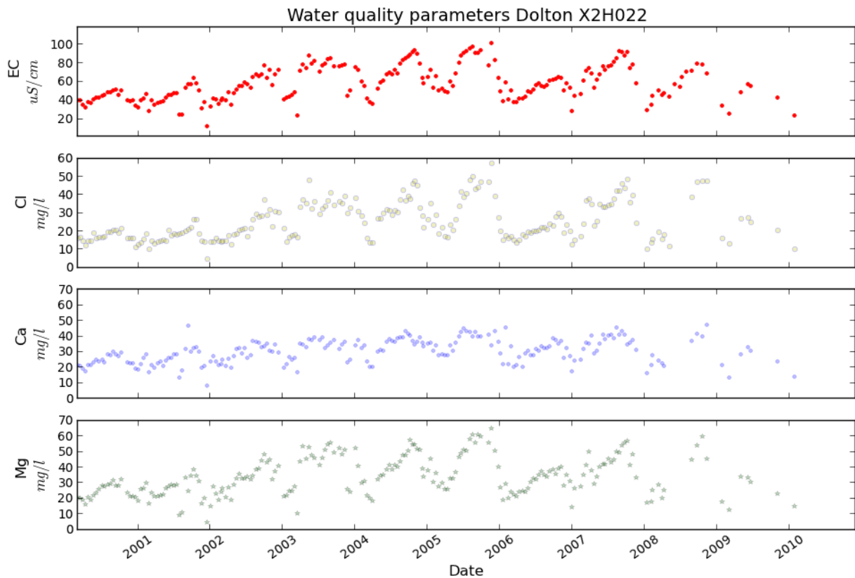
Figure 2.10: Long term variation of water quality parameters at Kaap outlet
