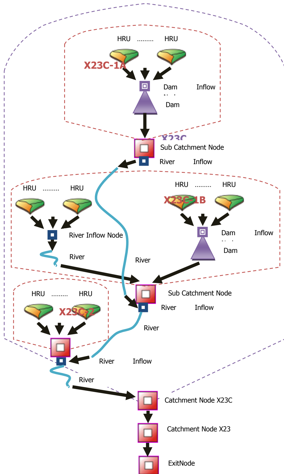
Figure 2.22: Configuration of the ACRU model for quaternary X23C
