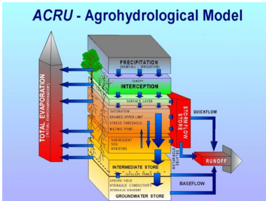
Figure 2.20: Multi-layer soil water budgeting through the partitioning and redistribution of soil water (Schulze, 1995).
