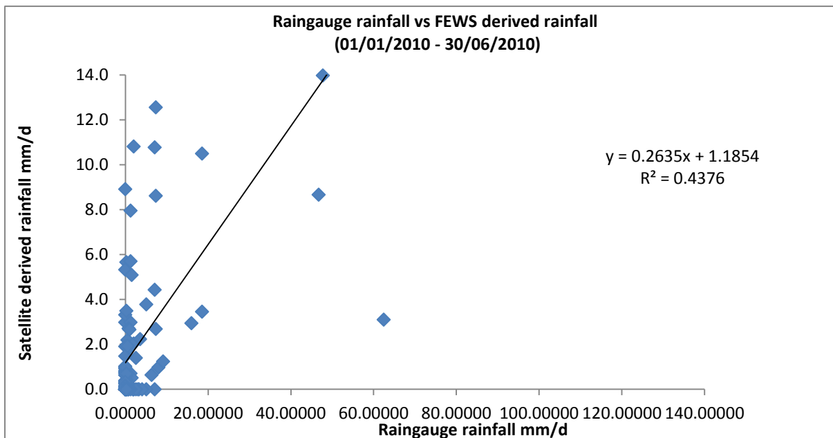
Figure 2.25: R^2 for Raingauge versus FEWS rainfall
