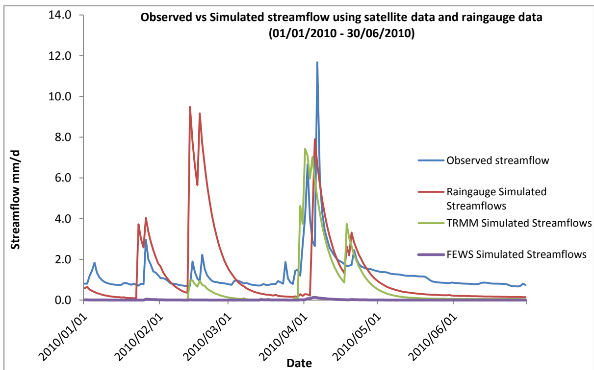
Figure 2.26: Comparison of Simulated streamflows for raingauge, TRMM and FEWS datasets.
