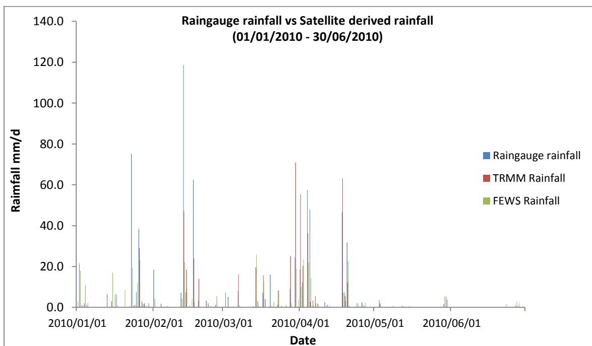
Figure 2.23: Comparison between raingauge, TRMM and FEWS rainfall estimates
