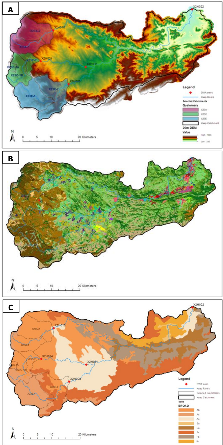
Figure 2.21: The Kaap Catchment (A – quaternary catchments with the 20 m DEM; B - Newly derived Landcover; and C - Soils information).
