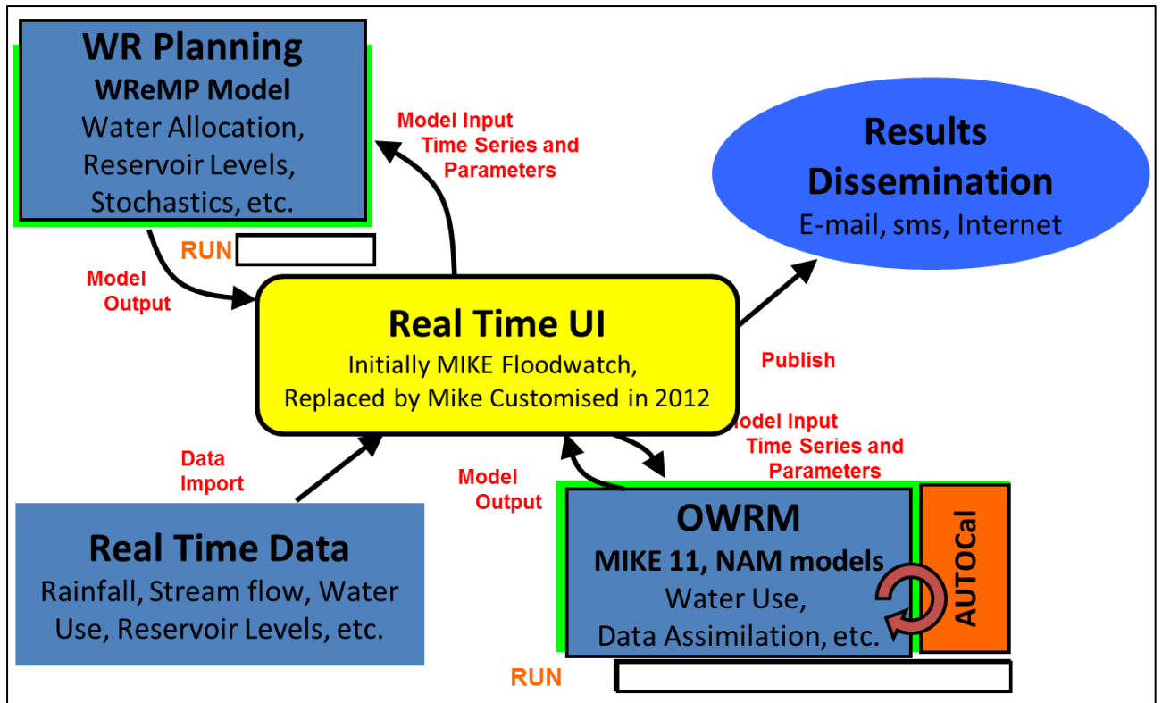
Figure 3.3: Conceptual Representation of the Operational Water Resources Management Decision Support System implemented in the Crocodile Catchment (Hallowes et al., 2007), where the WReMP is the long term water resources planning model and the MIKE suite of tools integrates this and other information for real-time operations for the Crocodile River (for further detail see Appendix II ).
