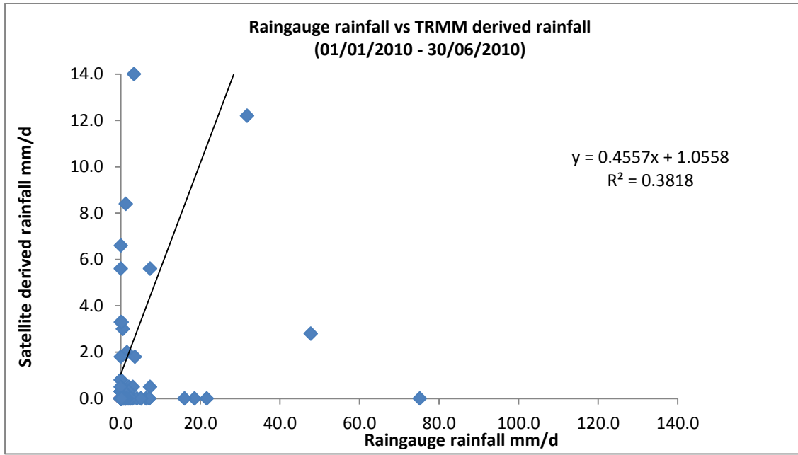
Figure 2.24: R^2 for Raingauge versus TRMM rainfall
