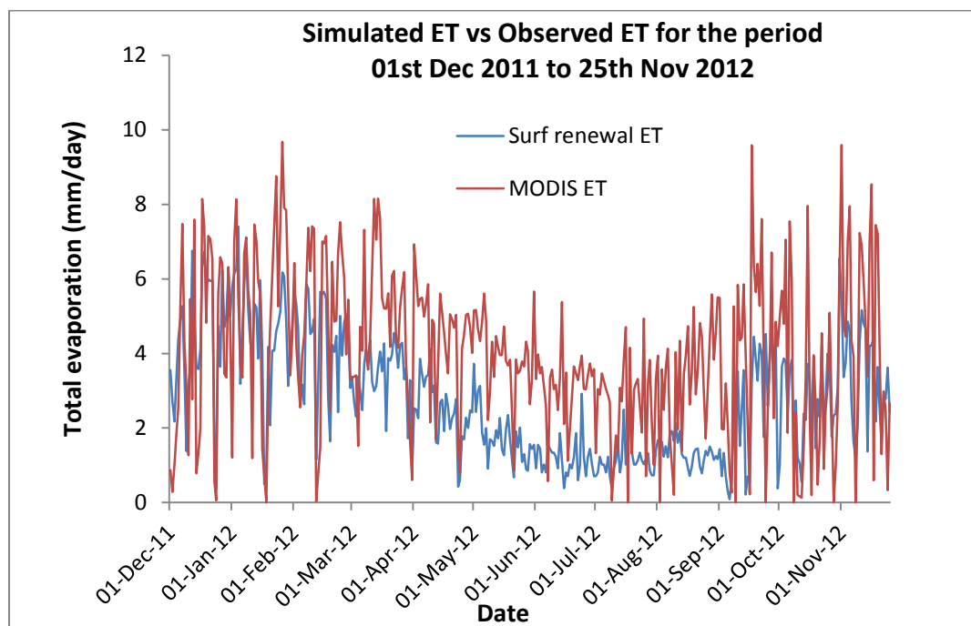
Figure 2.17: comparison between SEBS daily total evaporation estimates and Surface renewal daily total evaporation estimates
