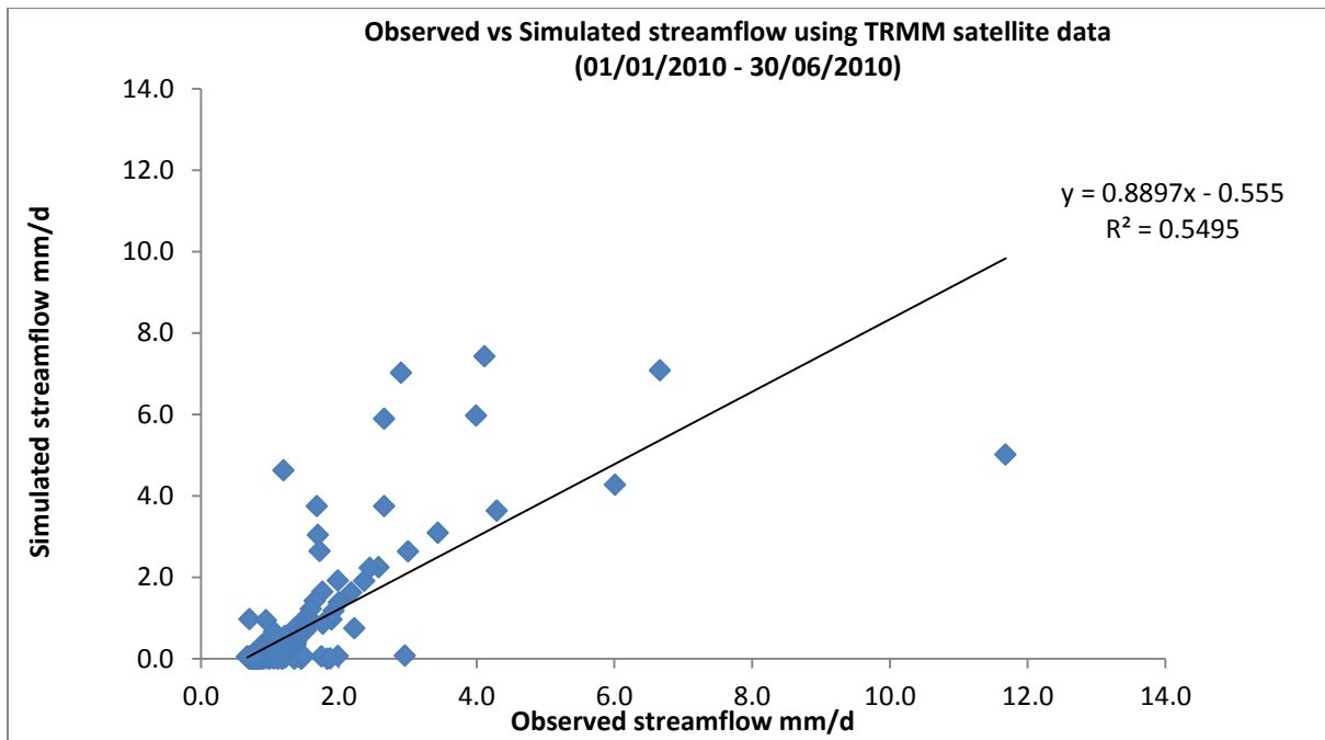
Figure 2.27: Comparison of Simulated streamflows from rain gauge versus TRMM datasets.
