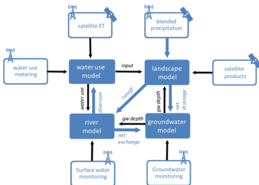
Figure 2.12: Conceptual framework of the AWRA system (van Dijk and Renzullo, 2011)
