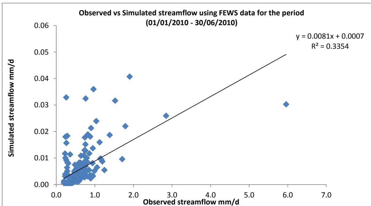
Figure 2.28: Comparison of Simulated streamflows from rain gauge versus FEWS datasets.
