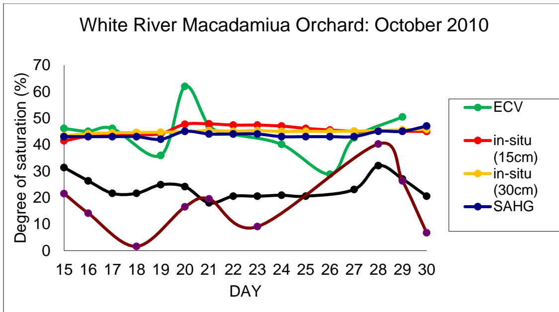
Figure 2.19: Soil Moisture Measurements for different products (October 2010) at White River
