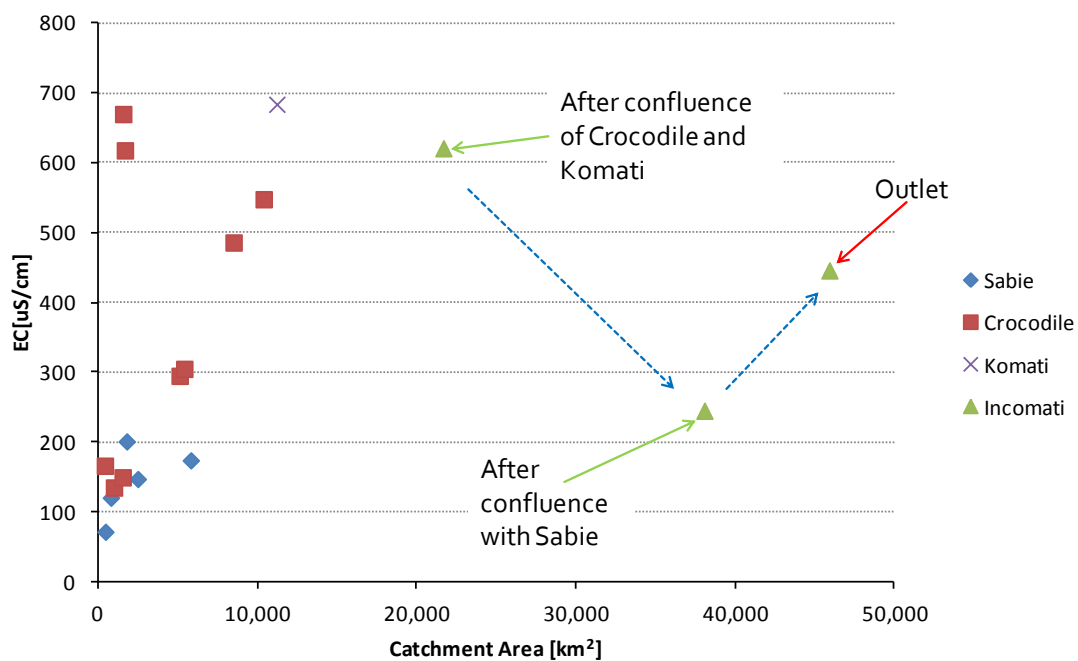
Figure 2.9: Scaling effects of EC in function of the drainage area, for the main sub-catchments of Incomati
