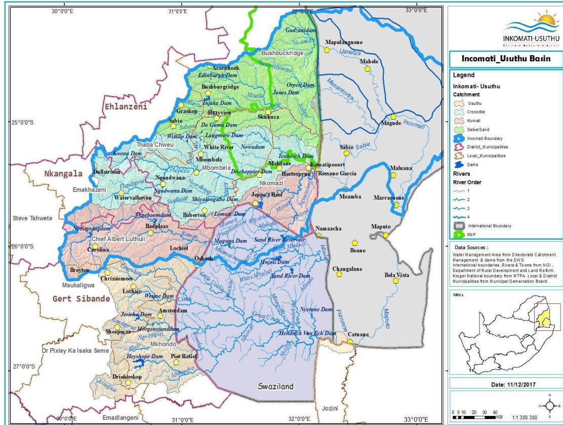
Figure 1: Map of the Inkomati-Usuthu Water Management Area.
